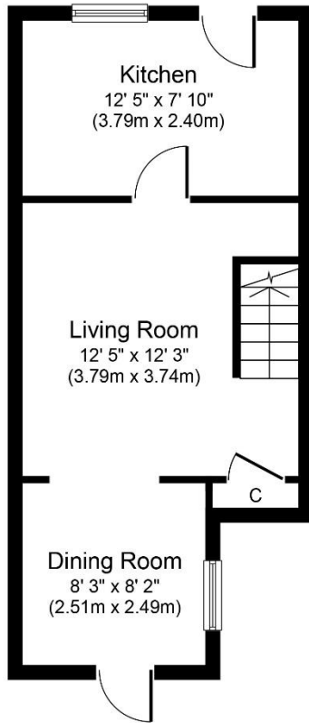
Ground Floor Approximate Floor Area 330 sq. ft. (30.7 sq. m.)
